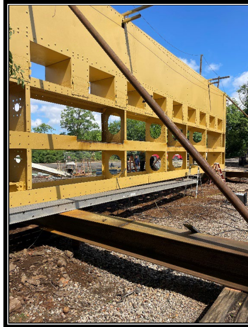
Figure 2: East Tide Gate primed.
