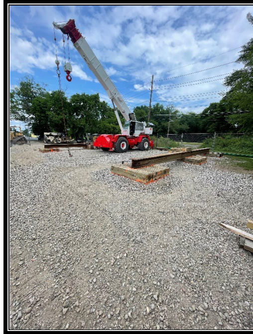
Figure 2: Driscoll Construction completing staging to support tide gate.
