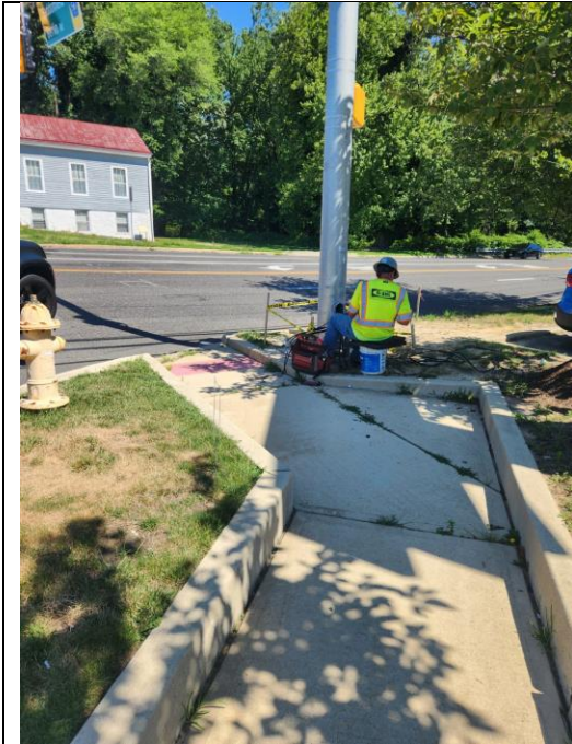
Photo B-1 of 1 Date Taken: July 2, 2024 Description: DIEHL continues signal cable work (P.S 11 OF 16 Electrical Plan)
