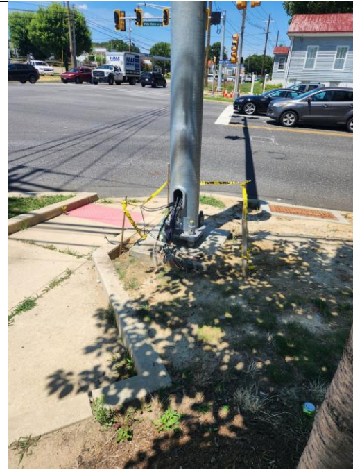
Photo B-2 of 2 Date Taken: July 2, 2024 Description: DIEHL continues signal cable work) (P.S 11 OF 16 Electrical Plan)
