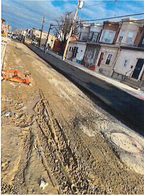
Figure 2: Paving HMA Base Course
