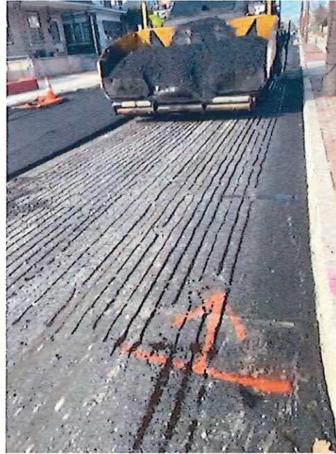
Figure 3: Applied Tack Coat
