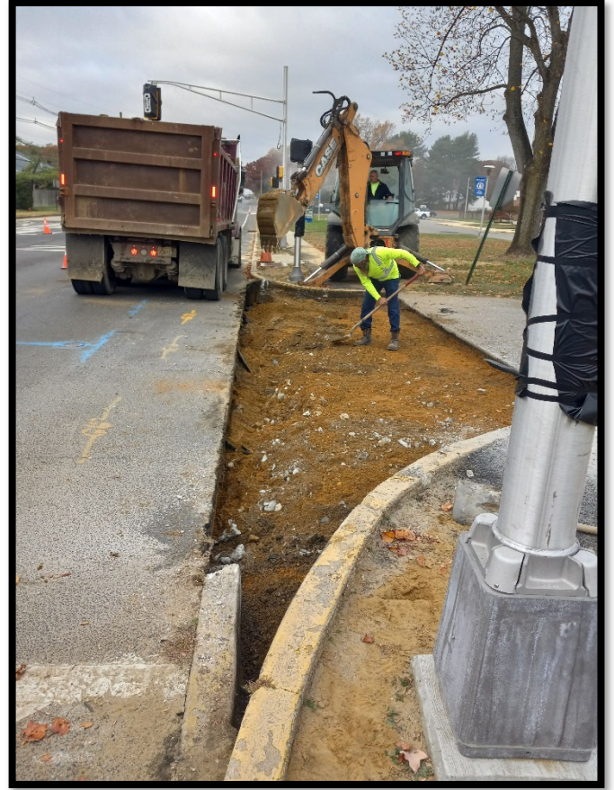
Photograph 4 – Concrete crew preparing for driveway apron installation at entrance to Cooper Elementary School.
