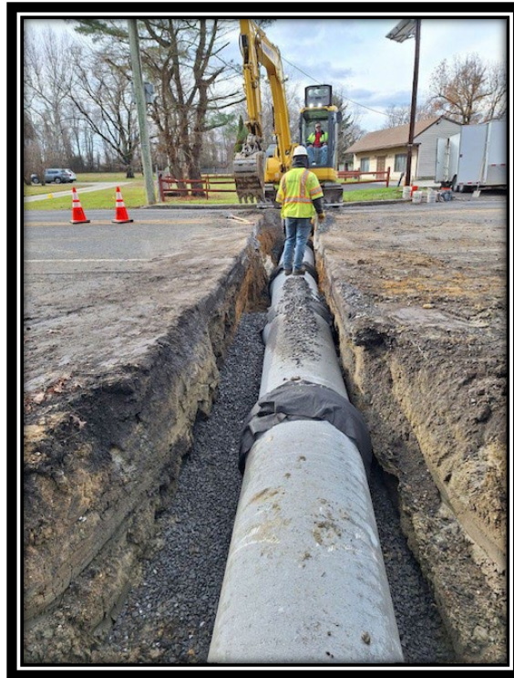
Figure: 2 – Installation of 24” RCP crossing between Tall Oaks Drive and Mt. Pleasant Road
