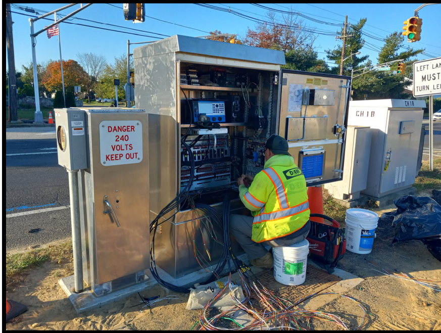
Photograph 7 – Electrical subcontractor making electrical connections in the new traffic signal control box at the S. Birchwood Park Drive intersection.
