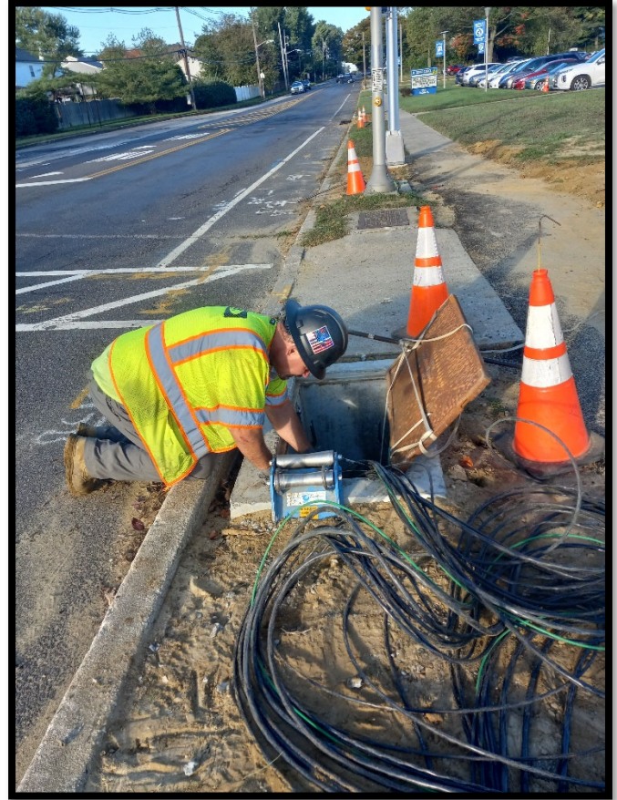
Photograph 4 – Electrical subcontractor pulling wires for the new traffic signal at S. Birchwood Park Drive intersection.
