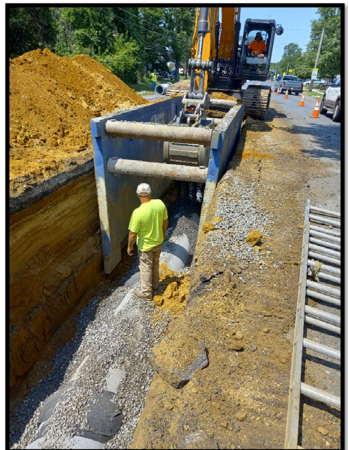
Photograph 2 – Pipe subcontractor installing 30" RCP storm pipe.
