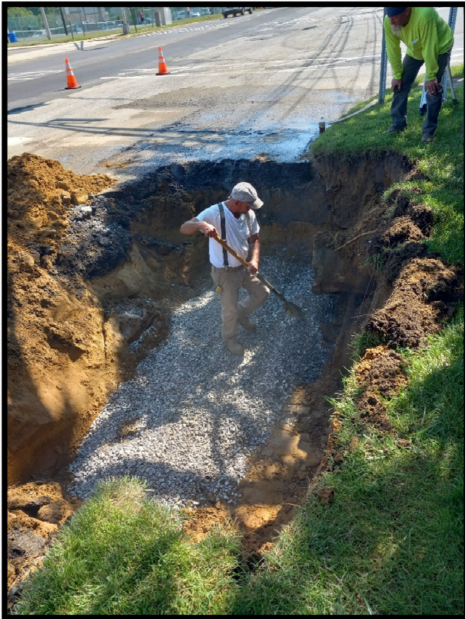
Photograph 1 – Deteriorated Existing “B” Inlet removed at Station 138+75R in preparation for installation of new precast Double “B” Inlet.
