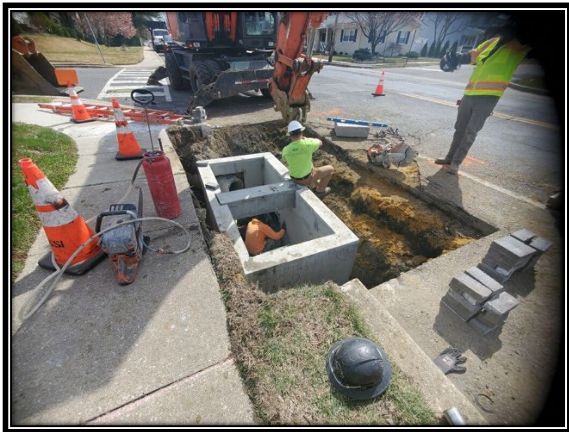
Figure: 1 – Installation of Type Double B Inlet along the northbound lane at the intersection with Maple Avenue
