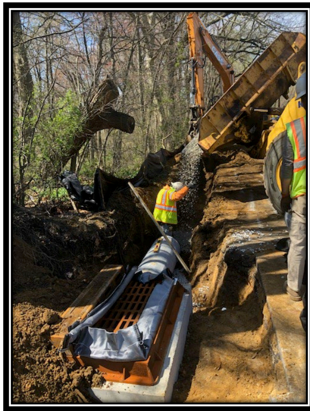
Figure: 1 – Installation of 15” RCP along the eastbound lane between Kings Croft Drive and the County Border
