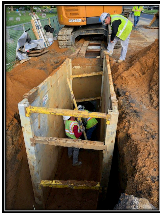
Figure: 1 – Connection of 18” RCP into a newly installed Double B Inlet along the eastbound lane between Millstream Drive and Friendship Lane
