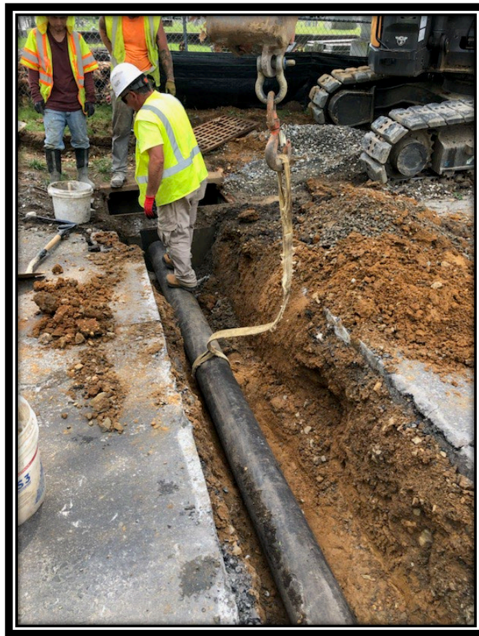
Figure: 1 – Installation of 12” DIP storm sewer at the intersection with Friendship Lane
