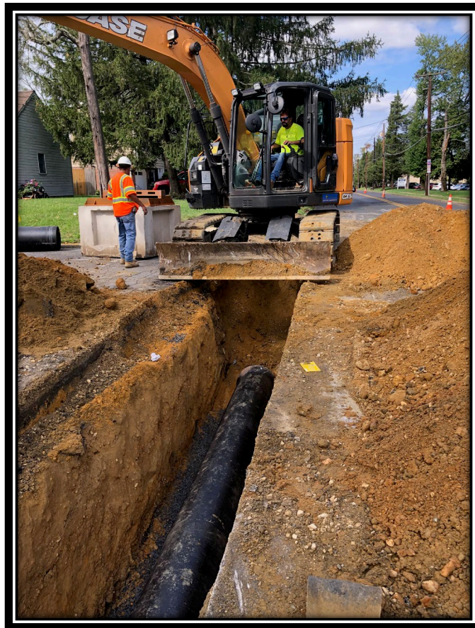
Figure: 1 – Installation of 18” DIP along the eastbound lane at the intersection with West Lake Drive
