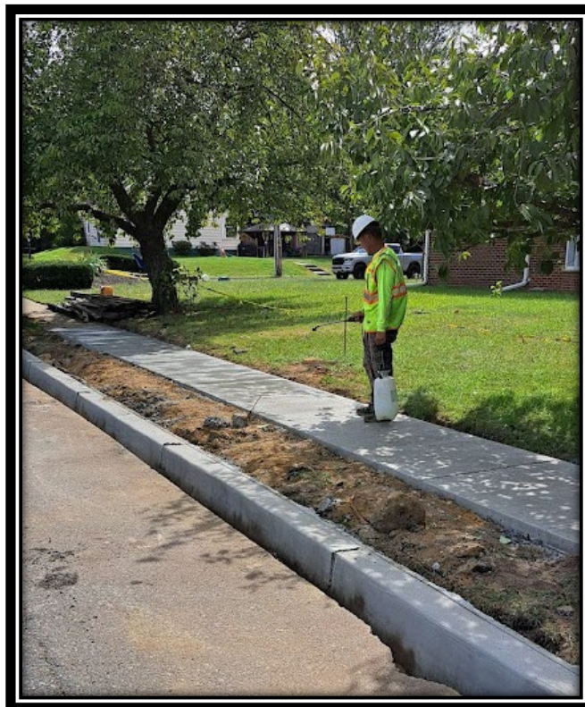
Figure: 3 – Spraying of curing compound on newly installed concrete curb and sidewalk along the eastbound lane between Wilson Road and Columbia Boulevard
