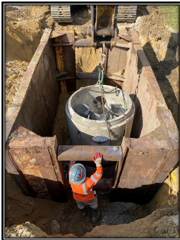
Figure: P&A Construction installing the final Dual Vortex Separator Unit.
