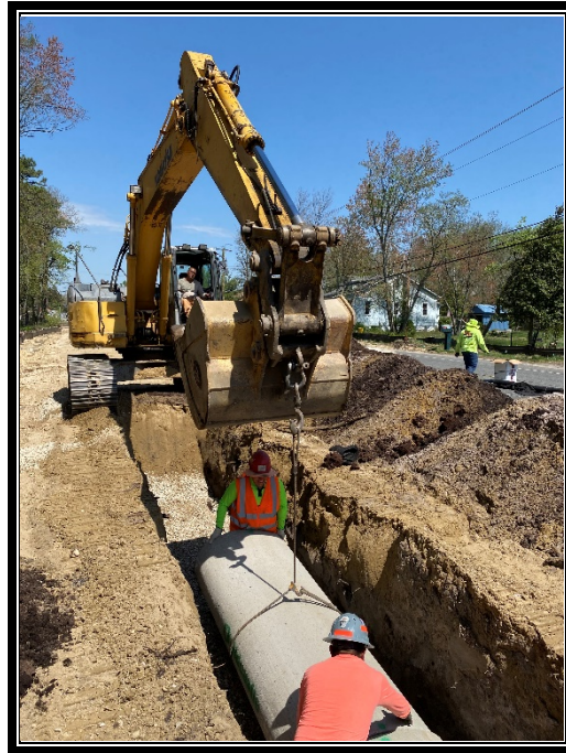
Figure 2: P&A Construction installing reinforced concrete pipe.
