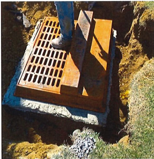
Figure 4: Inlet frame and grate
