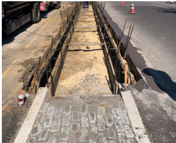
Figure 2: Concrete restraint curb forms
