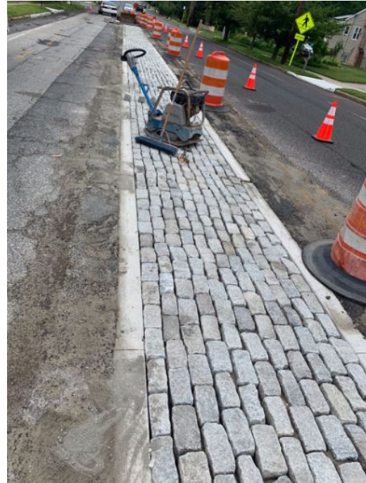
Figure 5: Concrete island pavers installed
