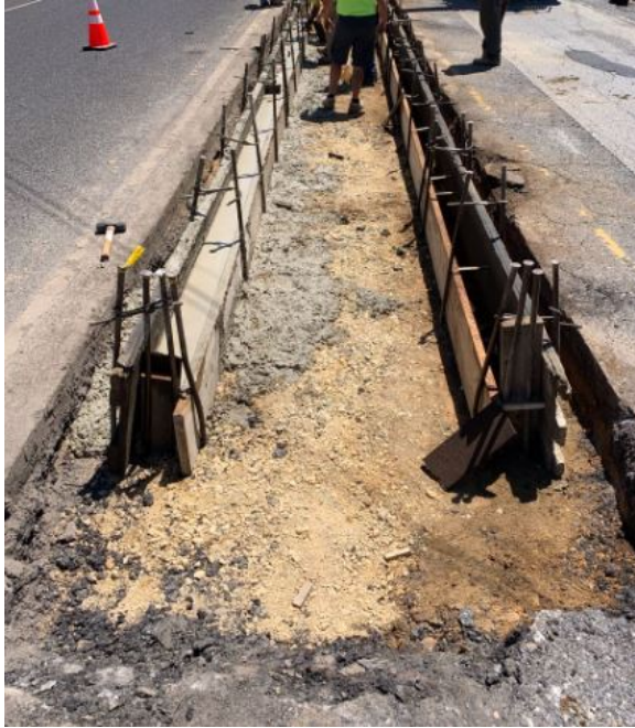
Figure 4: Concrete curb restraint placed
