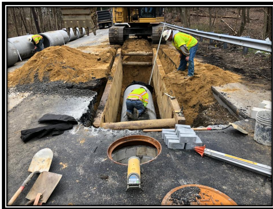
Figure: 3 – Installation of 36" RCP along the southbound lane of Watsontown-New Freedom Road (CR 691) between Berlin-Clementon Road and Carriage Stop Drive in the Borough of Pine Hill
