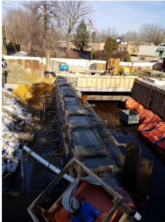
West wing wall after concrete is poured
