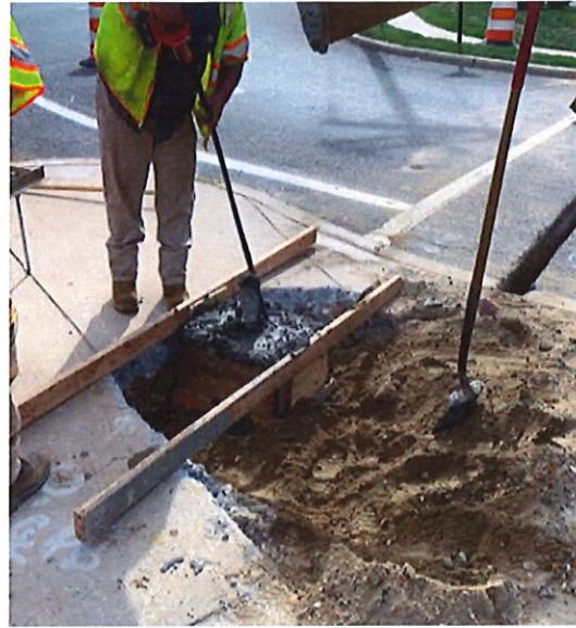
Figure 3: Pouring pedestal foundation
