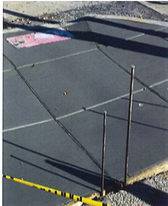
Figure 5: ADA curb ramp and sidewalk
